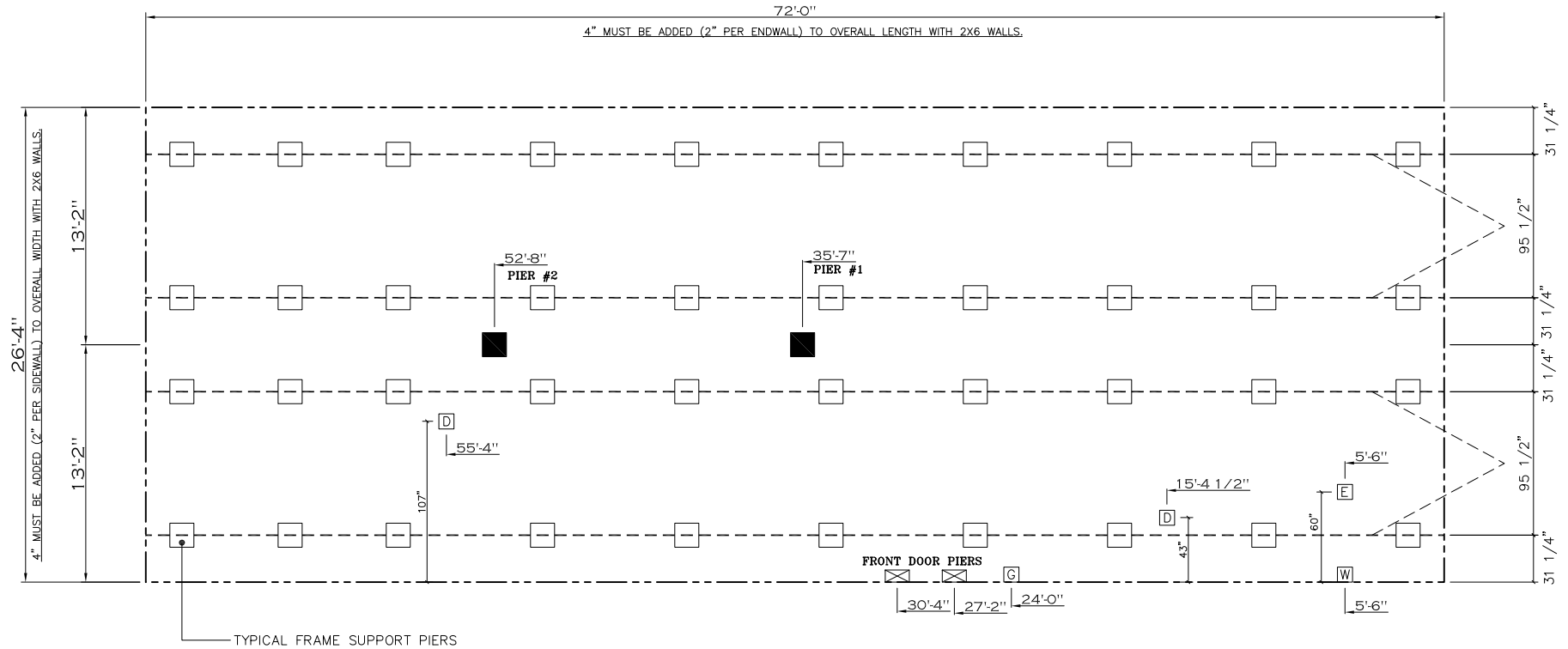
TYPICAL FRAME SUPPORT PIERS
