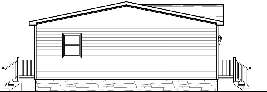
LEFT ELEVATION
